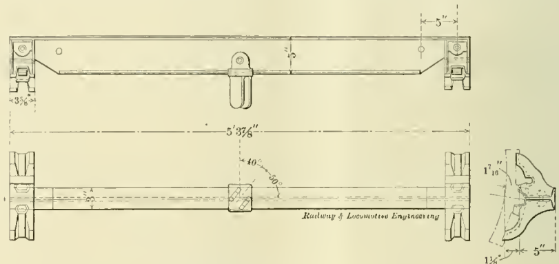
VANDERBILT STEEL BRAKE BEAM.
